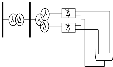
Fig. 8 Structure 03 of a DC EAF
