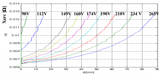
Fig. 10 Variation of Xarc
