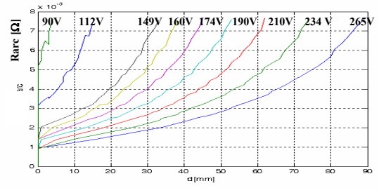
Fig. 11 Variation of Rarc
