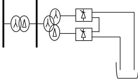
Fig. 7 Structure 02 of a DC EAF
