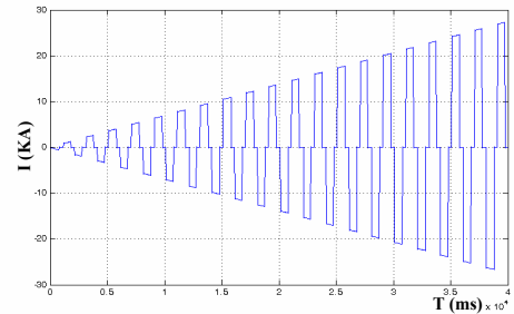
Fig. 3 Current at the star of transformer rectifier
