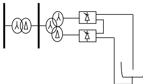
Fig. 9 Structure 04 of a DC EAF
