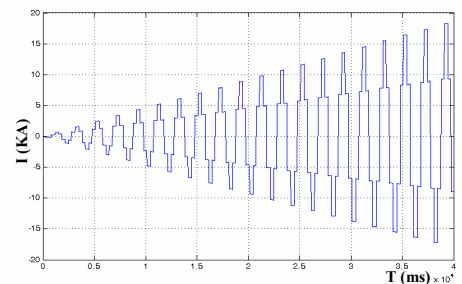
Fig. 4 Current at the triangle of transformer rectifier
