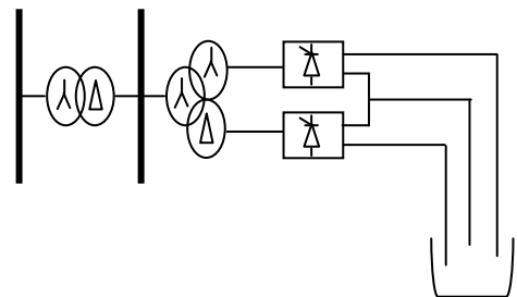
Fig. 6 Structure 01 of a DC EAF
