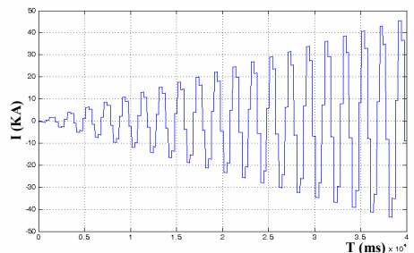
Fig. 5 Current of twelve pulse rectifier
