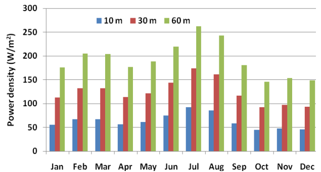
Fig. 4. Monthly extrapolation of Power density
