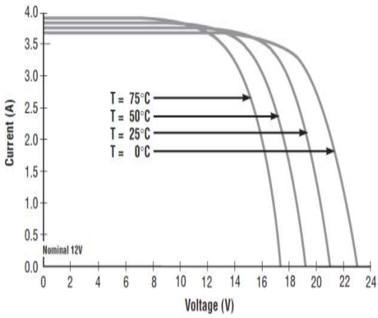
Fig. 3. The MSX-60 PV module I-V characteristic of the manufacturer.
