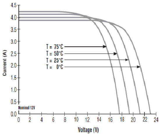
Fig. 5. The MSX-64 PV module I-V characteristic of the manufacturer.
