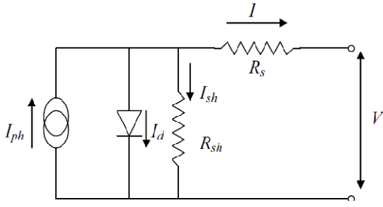
Fig. 1: Equivalent circuit of a single diode model.
