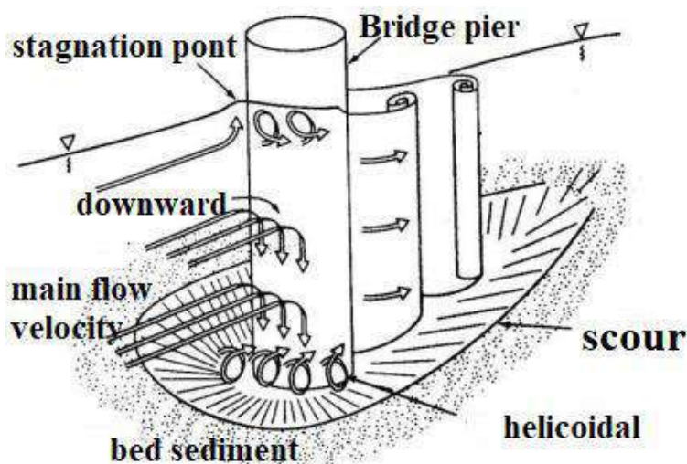
Fig.1 flow patterns around the cylindrical bridge pier
