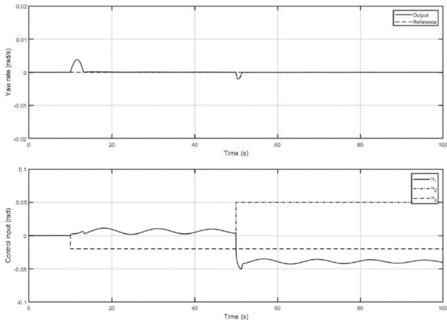
Figure 1: Stabilization of the yaw rate with 2 actuator failures
