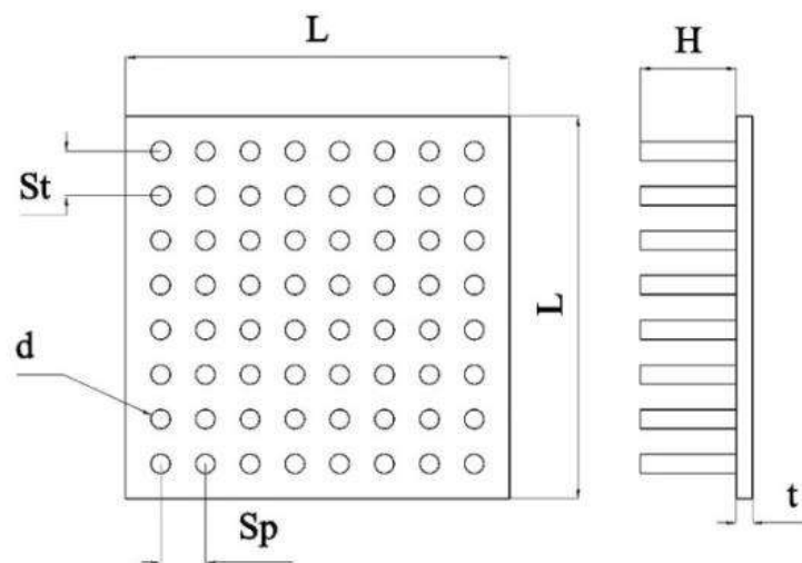
Figure 1. Details of heat exchanger pin plates
