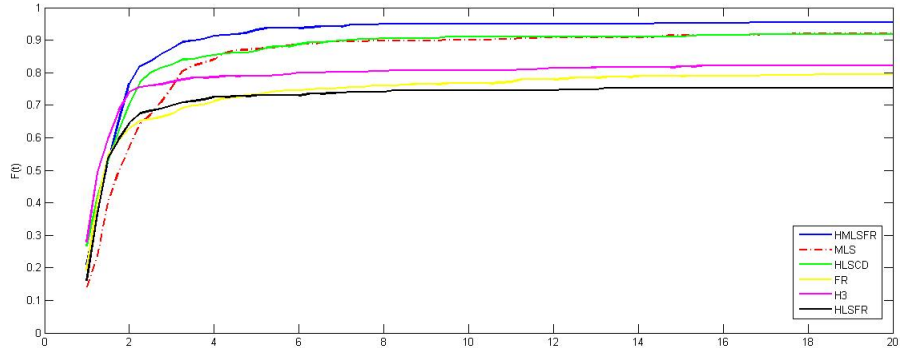
Figure 2. Performance profile based on the CPU time
